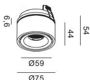
Glow 59 Recessed
