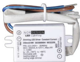
Nordesign LED driver - 4W/350mA (6-12V) Art. nr. 303500004 Elnr. 6632259
